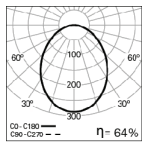
VEGA IP D95 LIGHT+ 4000K HO
