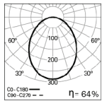
VEGA D95 LIGHT+ 4000K HO
