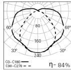
STELLA 66 L1277W145 DC0 4000K
