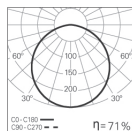
ROFY LED 105W DOZ 4000K
