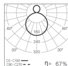
ROFY D/I LED 159W DOZ 4000K
