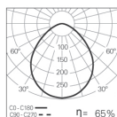
ROFY Z LED 68W gCONTROL+ 4000K
