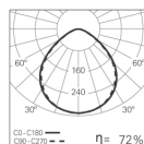
ROFY Z LED 47W gCONTROL 4000K
