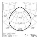
ROFY LED 36W gCONTROL 4000K
