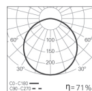
ROFY /E LED 105W DOZ 4000K
