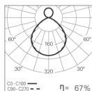
ROFY D/I LED 72W gCONTROL 4000K
