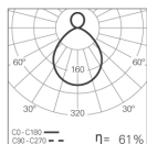
ROFY D/I LED 103W gCONTROL 4000K
