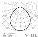
ROFY LED 68W gCONTROL+ 4000K
