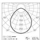
ROFY /E LED 68W gCONTROL 4000K
