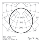
ROFY Z LED 105W DOZ 4000K
