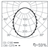
REBA/E LED 39W bLINE 4000K
