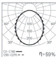
REBA LED 39W bLINE 4000K
