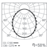
REBA /T LED 47W bLINE 4000K
