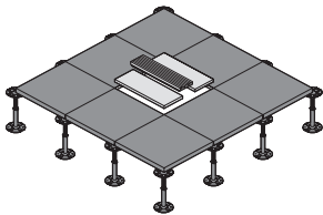
GRS/150 GRS/300 GRS/600 aluminium ventilation grid with dumper for air regulation
